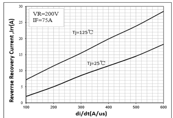
Fig.4 Reverse Recovery Current vs dI_F/dt
